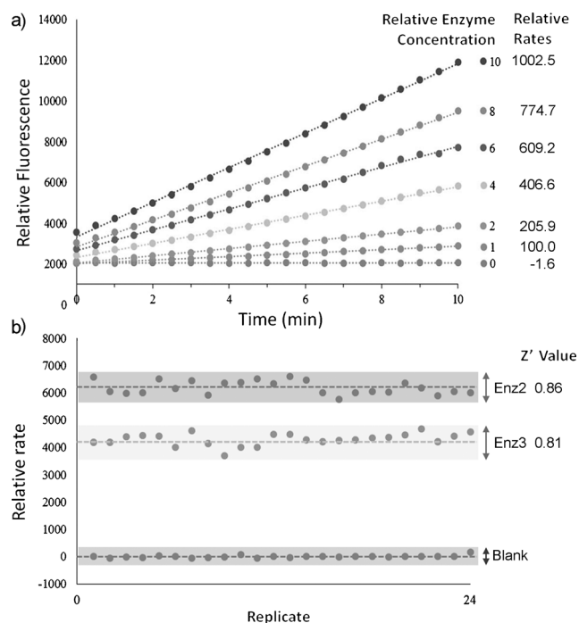
Figure 4. Detection of the enzymatic activities of endoglycoceramidase (Enz2) from Rhodococcus strain M-777 and neuraminidase (Enz3) from Micromonospora viridifaciens in cell lysates. a) Dependence of rate upon crude lysate concentration. Changes in fluorescence upon the addition to 1 of 0 \mu L, 5 \mu L, 10 \mu L, 20 \mu L, 30 \mu L, 40 \mu L or 50 \mu L of 100 \times diluted crude lysate from E. coli cells expressing Enz3. The relative amounts of enzyme and relative reaction rates are shown. b) Reproducibility of the assay when using probe 1 . Crude lysate from E. coli cells expressing Enz2 or Enz3 was added to 1 in buffer in a 96-well plate. Lysate from E. coli BL21 (DE3), which carries an empty pET28a plasmid, was used as a blank.
