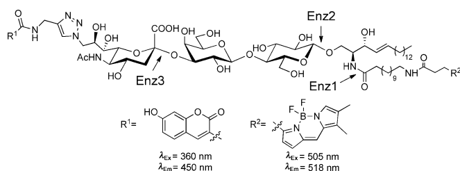
Figure 1. FRET probe 1 and its enzymatic cleavage points. The 7-hydroxycoumarin ( R^1 ) FRET donor is attached to the C9 position of sialic acid while the BODIPY FRET acceptor is attached to the terminus of the fatty acid alkyl chain. Enzymatic hydrolysis of the substrate by either sphingolipid ceramide N-deacylase (Enz1), endoglycosceramidase (Enz2), or neuraminidase (Enz3) will disrupt FRET. The arrows indicate where each enzyme cleaves the substrate.
