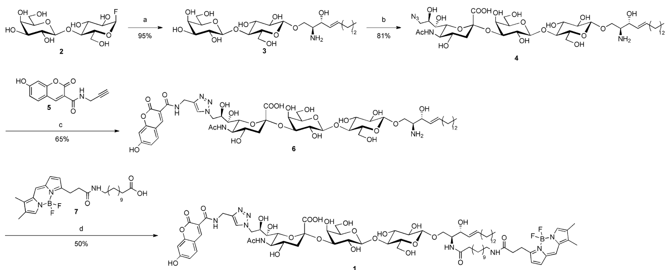
Scheme 1. Assembly of FRET probe 1 . a) EGCase glycosynthase, D-erythro-sphingosine, NaOAc buffer pH 5.3, 10% dimethoxyethane, 37 °C; b) CMP-9-azido-9-deoxy-sialic acid, \alpha 2,3-sialyltransferase, alkaline phosphatase, 50 mM Tris buffer (pH 7.5) containing 100 mM \text{MgCl}_2 , RT; c) alkyne coumarin 5 , 50 mM BTES buffer, 200 mM sodium ascorbate, 50 mM \text{CuSO}_4 , 50% DMF, 35 °C; d) BODIPY carboxylic acid 7 , SCDase glycosphingolipid N-deacylase, 50 mM HEPES buffer (pH 7.5), 10% dimethoxyethane, 35 °C.
