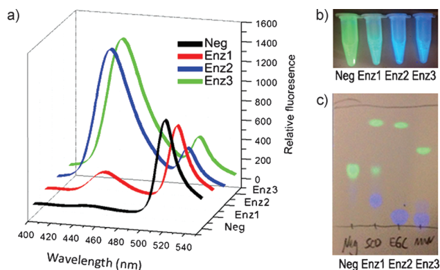
Figure 2. Hydrolysis of compound 1 by sphingolipid ceramide N-deacylase (Enz1), endoglycosidase (Enz2), or neuraminidase (Enz3). Addition of the enzymes to a 0.1 mM solution of probe 1 in 20 mM Tris-HCl buffer (pH 7.5) with 1 % Triton-X100 led to an increase in the coumarin fluorescence (blue) and a decrease in the BODIPY fluorescence (green). a) Fluorescence spectra before and after 30 min incubation with the different enzymes. b) Visual detection of the reactions under a UV lamp. c) Different hydrolysis patterns of probe 1 after hydrolysis by Enz1, Enz2, and Enz3. Neg: unreacted probe 1 as a negative control.
